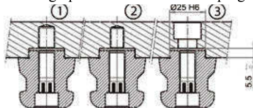
mounting options UNILOCK-clamping bolt
