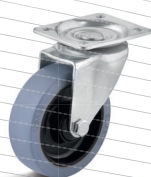
wheel ø 125 mm with grey rubber
