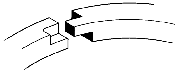
Design c Ring with single tenon
