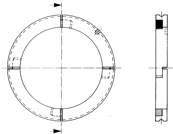
Fig. 15 Four piece carbon packing ring
