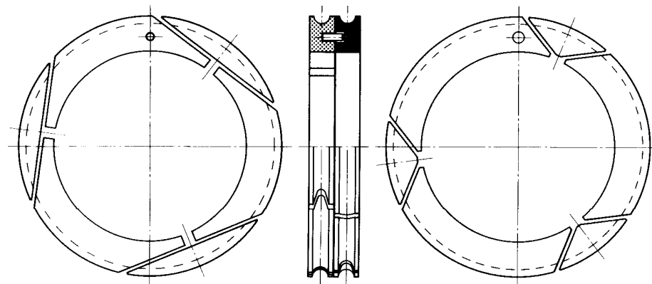
▲ Fig. 16 Carbon sealing rings with non-radially cut segment joints
