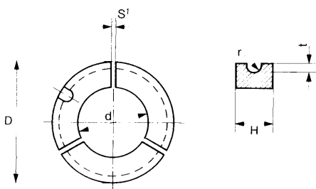
Fig. 14 Dimensioning of a ring and calculation of the garter tension spring
