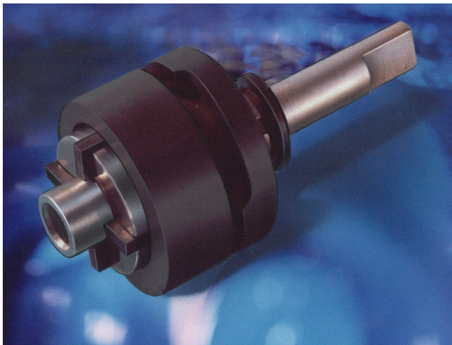
Fig. 17 Rotor Housing and Vanes of a Rotary Compressor
