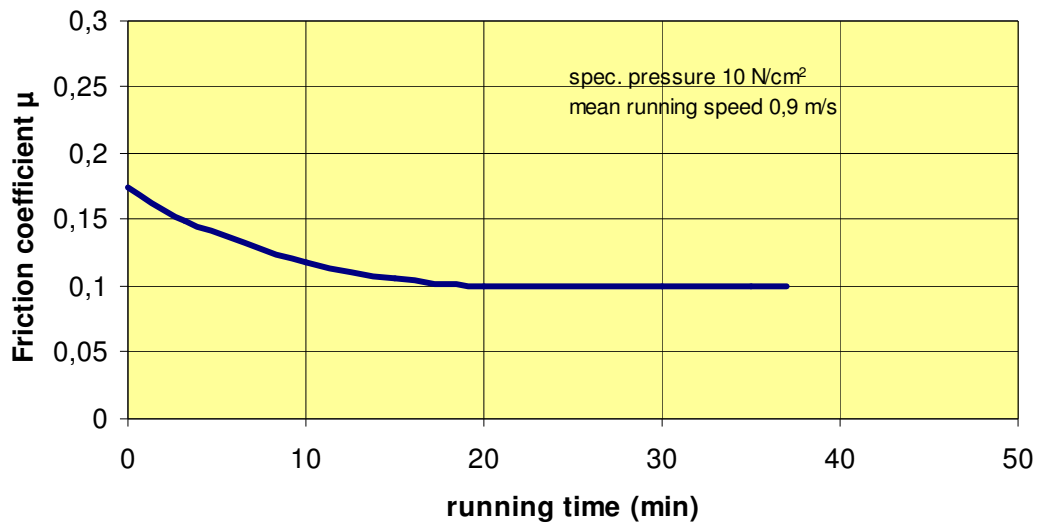
Fig. 1 Change of the friction coefficient \mu when running in
