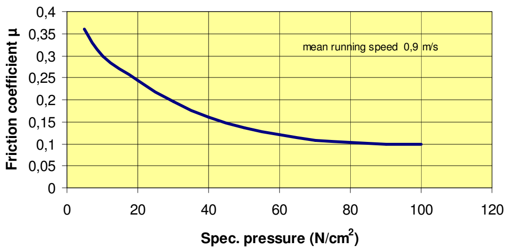
Fig. 3 Friction coefficient \mu dependent on the specific pressure
