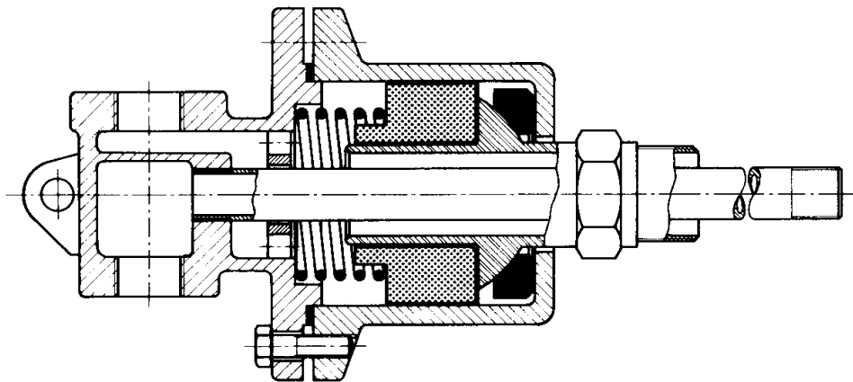
Fig. 9 Diagrammatic view of the installation of a carbon sealing ring in the heating joint of a calender drier.
