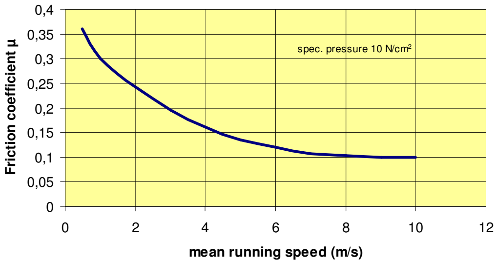
Fig. 2 Friction coefficient \mu dependent on the mean running speed
