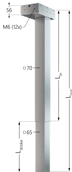
ELS3-500S-BTU-Q-HeavyDuty
