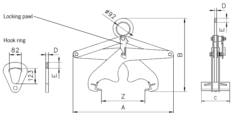
Model TPR, hook ring for grabs for 2000 kg and up capacity. Locking pawl locks open grab in place.
