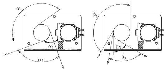
Rope lead-offs for pneumatic rope winch RPA
