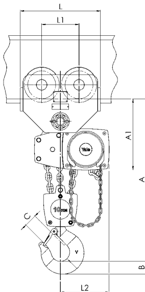
Model Yalelift ITG, 10000 kg, three fall
