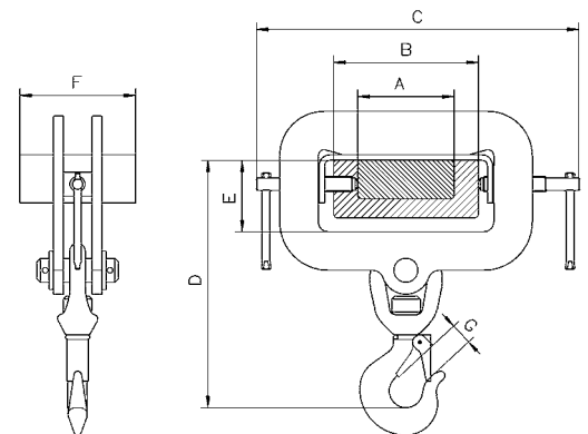
Model TZH, swivel hooks, pivoting and swivelling
