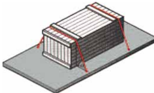
Applicable to textile lashings model ZGR-50-2500 with LC 2500 daN and model ZGR-50-2000 with LC 2000 daN
