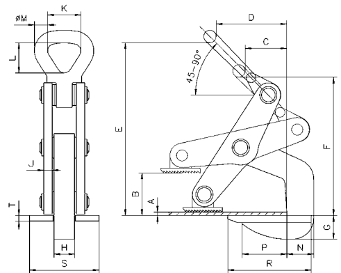
Model TWH with plate
