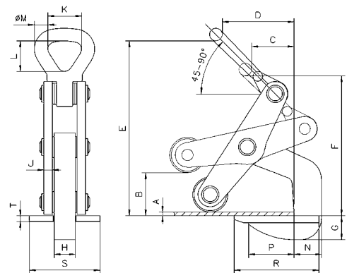
Model TWH with rollers
