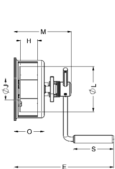
MWS, Capacity 300 - 600 kg
