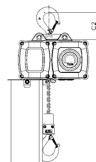
CPV/CPVF suspension hook, 250 - 2500 kg
