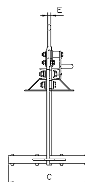
TBA 0.2-1t with serrated jaw
