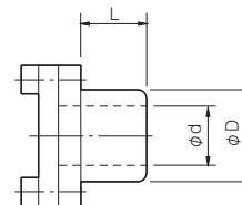
Figure B: Hub machining dimensions
